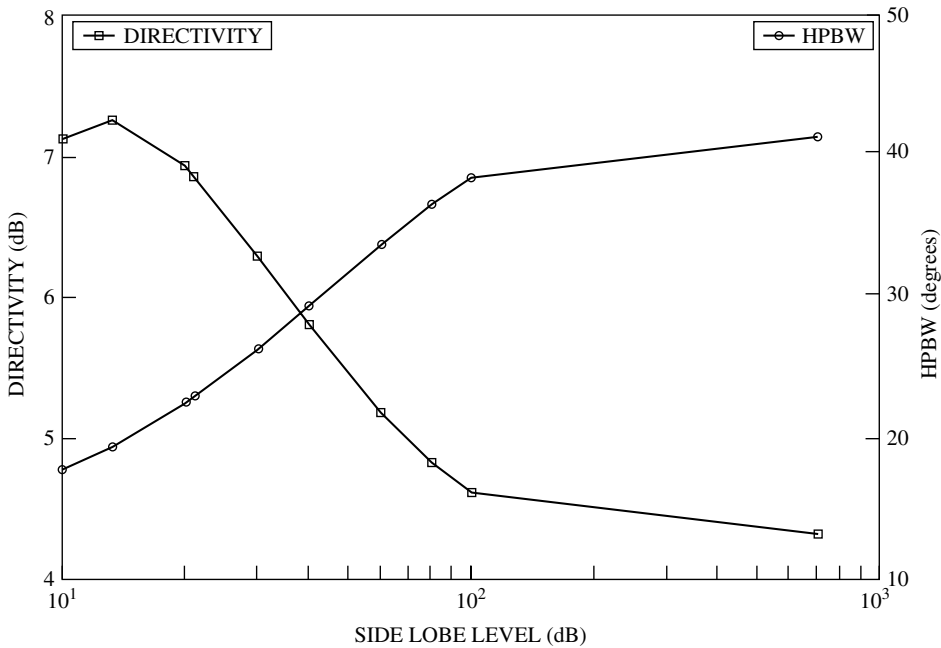
Figure 6.26 Directivity and half-power beamwidth versus side lobe level for a Dolph-Tschebyscheff array of N = 10 , d = \lambda/4 .
