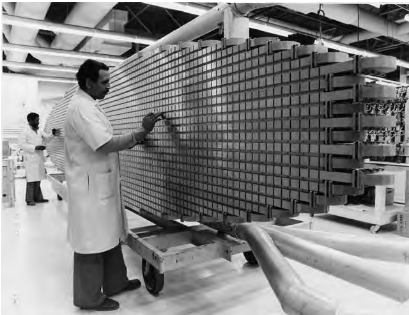
Figure 6.27 AWACS antenna array of waveguide slots. (PHOTOGRAPH COURTESY: Northrop Grumman Corporation).
