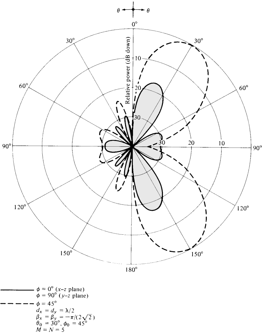
Figure 6.33 Two-dimensional antenna patterns of a planar array of isotropic elements with a spacing of d_x = d_y = \lambda/2 , equal amplitude, and progressive phase excitation.
