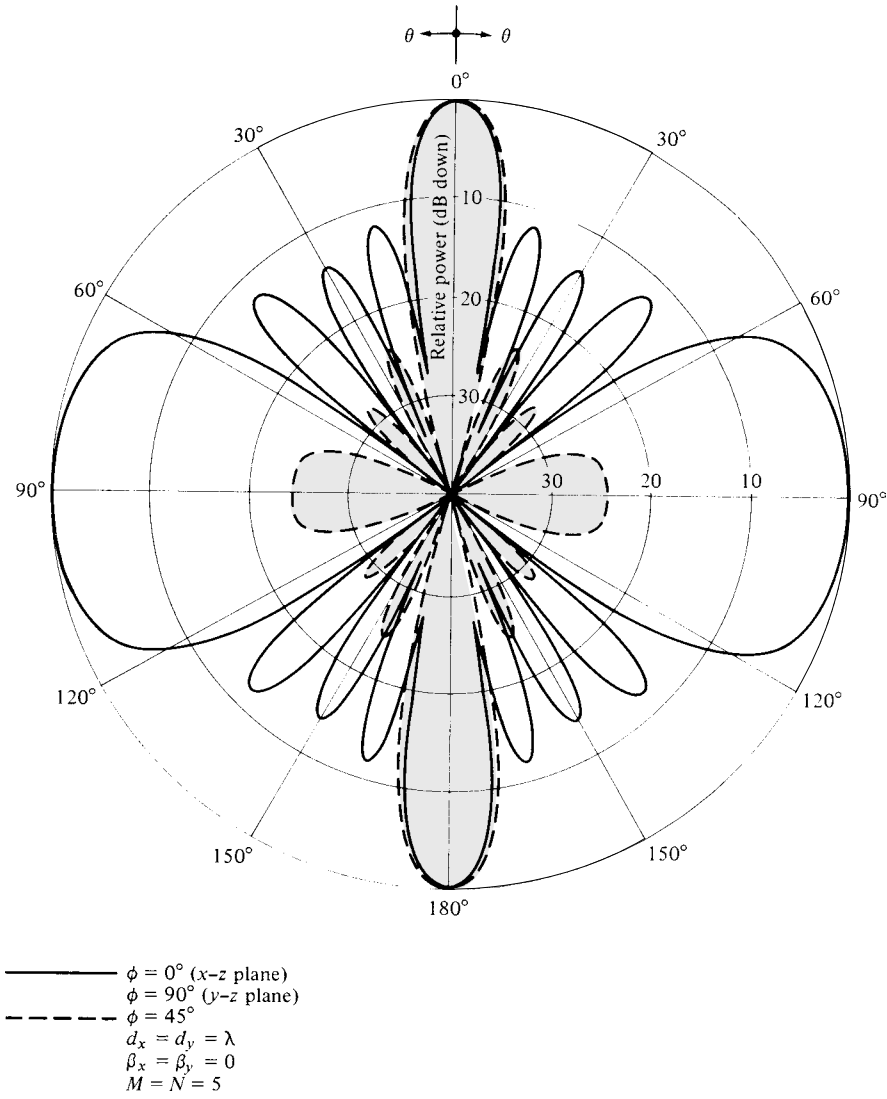
Figure 6.35 Two-dimensional antenna patterns of a planar array of isotropic elements with a spacing of d_x = d_y = \lambda , and equal amplitude and phase excitations.
