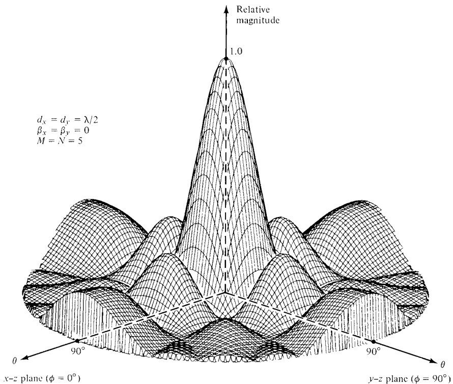
Figure 6.30 Three-dimensional antenna pattern of a planar array of isotropic elements with a spacing of d_x = d_y = \lambda/2 , and equal amplitude and phase excitations.
