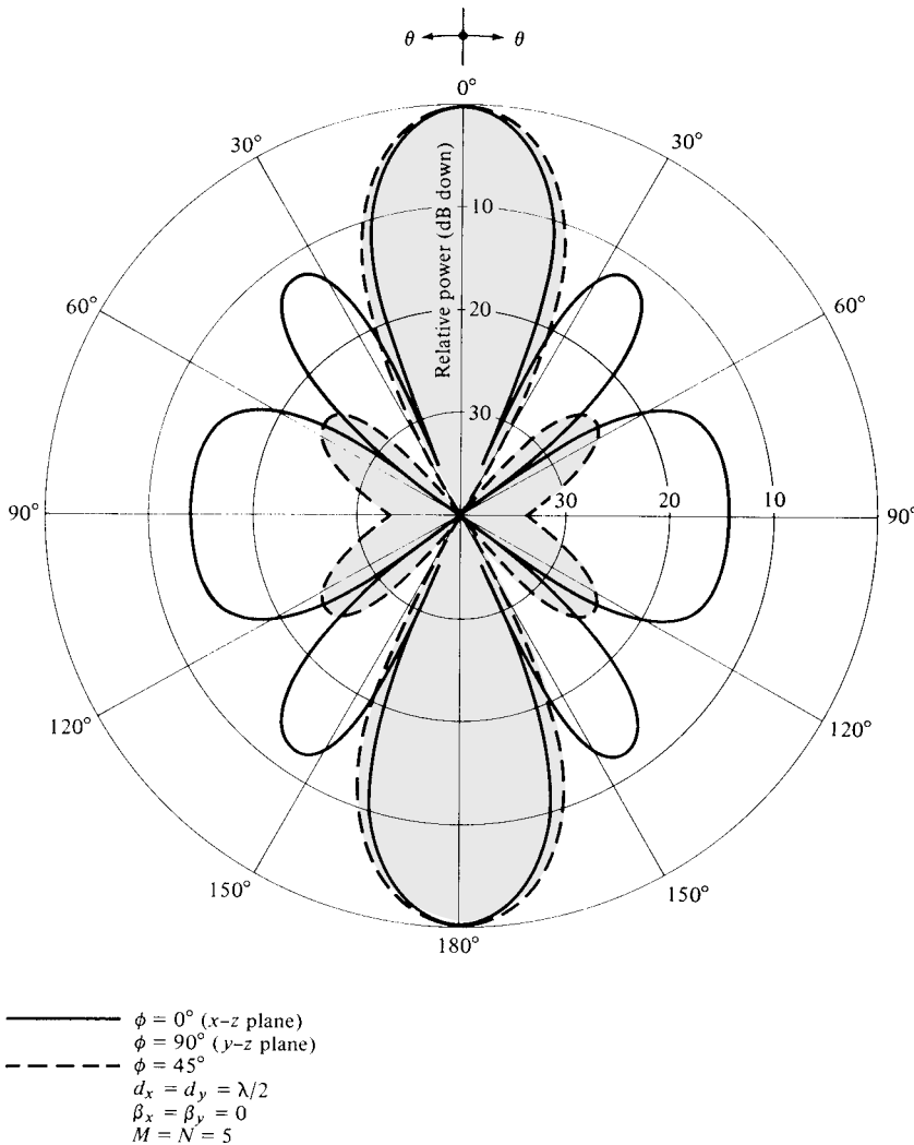
Figure 6.31 Two-dimensional antenna patterns of a planar array of isotropic elements with a spacing of d_x = d_y = \lambda/2 , and equal amplitude and phase excitations.
