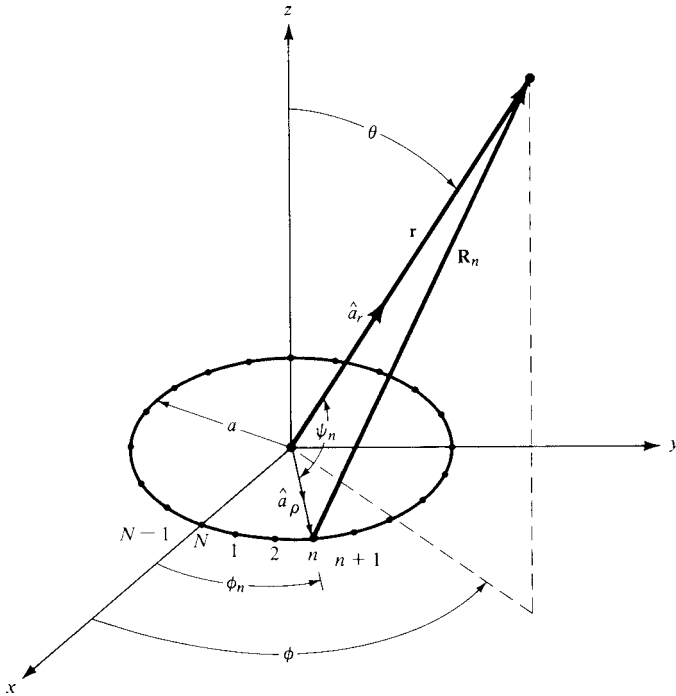
Figure 6.37 Geometry of an N -element circular array.
