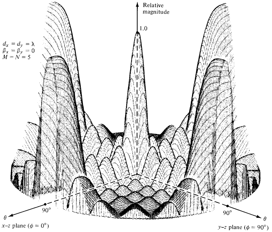
Figure 6.34 Three-dimensional antenna pattern of a planar array of isotropic elements with a spacing of d_x = d_y = \lambda , and equal amplitude and phase excitations.
