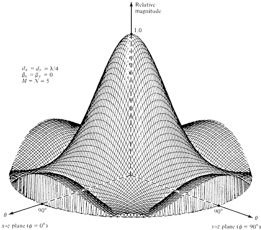
Figure 6.29 Three-dimensional antenna pattern of a planar array of isotropic elements with a spacing of d_x = d_y = \lambda/4 , and equal amplitude and phase excitations.
