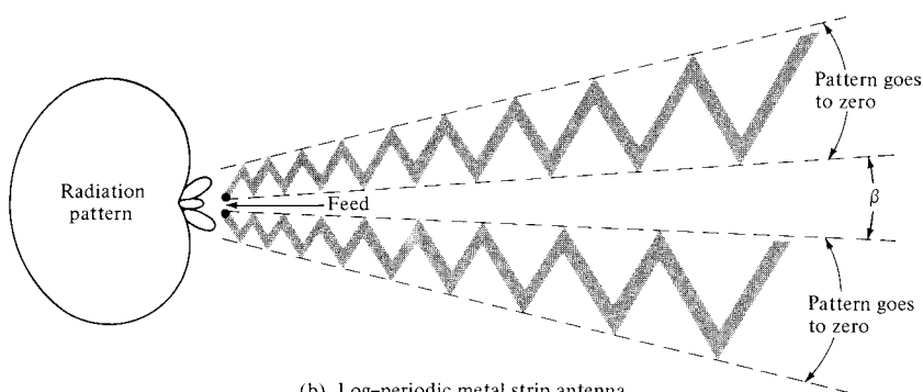
Figure 11.5 Typical metal strip log-periodic configuration and antenna structure.
