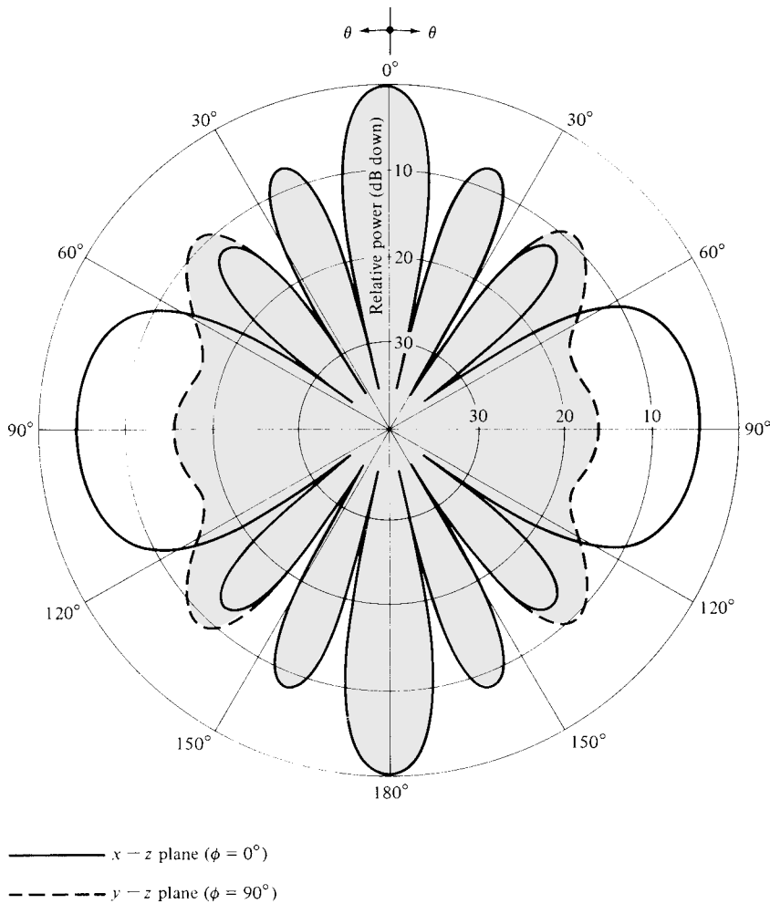
Figure 6.39 Principal-plane amplitude patterns of the array factor for a uniform circular array of N = 10 elements ( C/\lambda = ka = 10 ).
