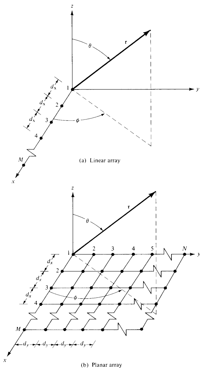
Figure 6.28 Linear and planar array geometries.
