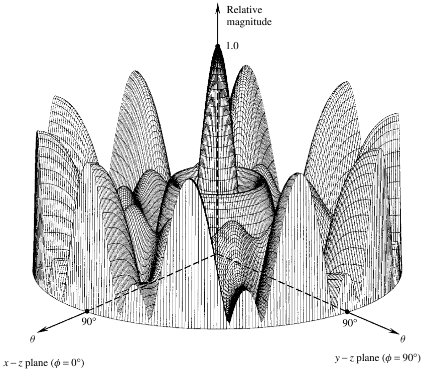
Figure 6.38 Three-dimensional amplitude pattern of the array factor for a uniform circular array of N = 10 elements ( C/\lambda = ka = 10 ).
