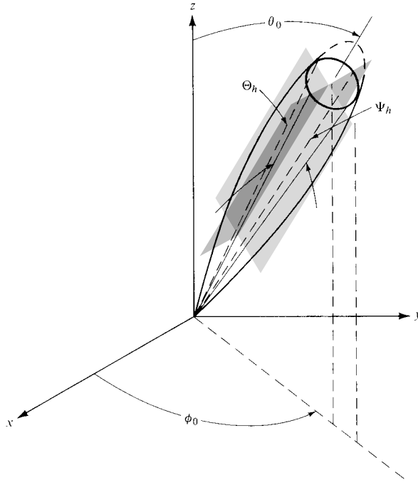
Figure 6.36 Half-power beamwidths for a conical main beam oriented toward \theta = \theta_0 , \phi = \phi_0 . (SOURCE: R. S. Elliott, "Beamwidth and Directivity of Large Scanning Arrays," Last of Two Parts, The Microwave Journal , January 1964.)
