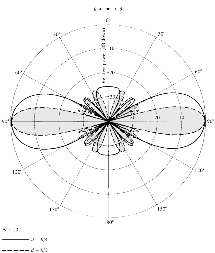
Figure 6.23 Array factor power pattern of a 10-element broadside Dolph-Tschebyscheff array.
