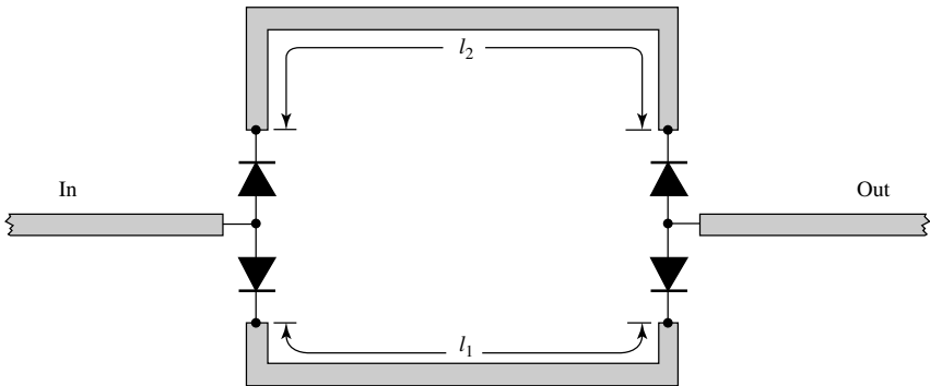
Figure 6.10 Incremental switched-line phase shifter using PIN diodes. (SOURCE: D.M. Pozar, Microwave Engineering , John Wiley & Sons, Inc. 2004).
