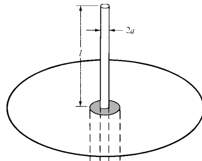
(a) Cylindrical monopole
