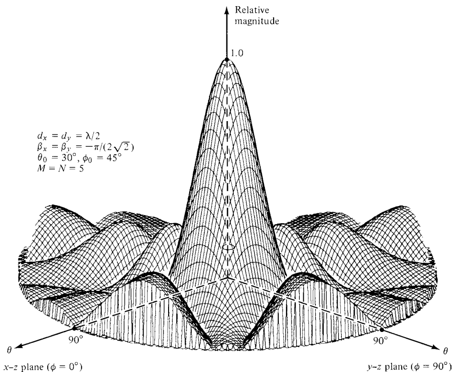
Figure 6.32 Three-dimensional antenna pattern of a planar array of isotropic elements with a spacing of d_x = d_y = \lambda/2 , equal amplitude, and progressive phase excitation.
