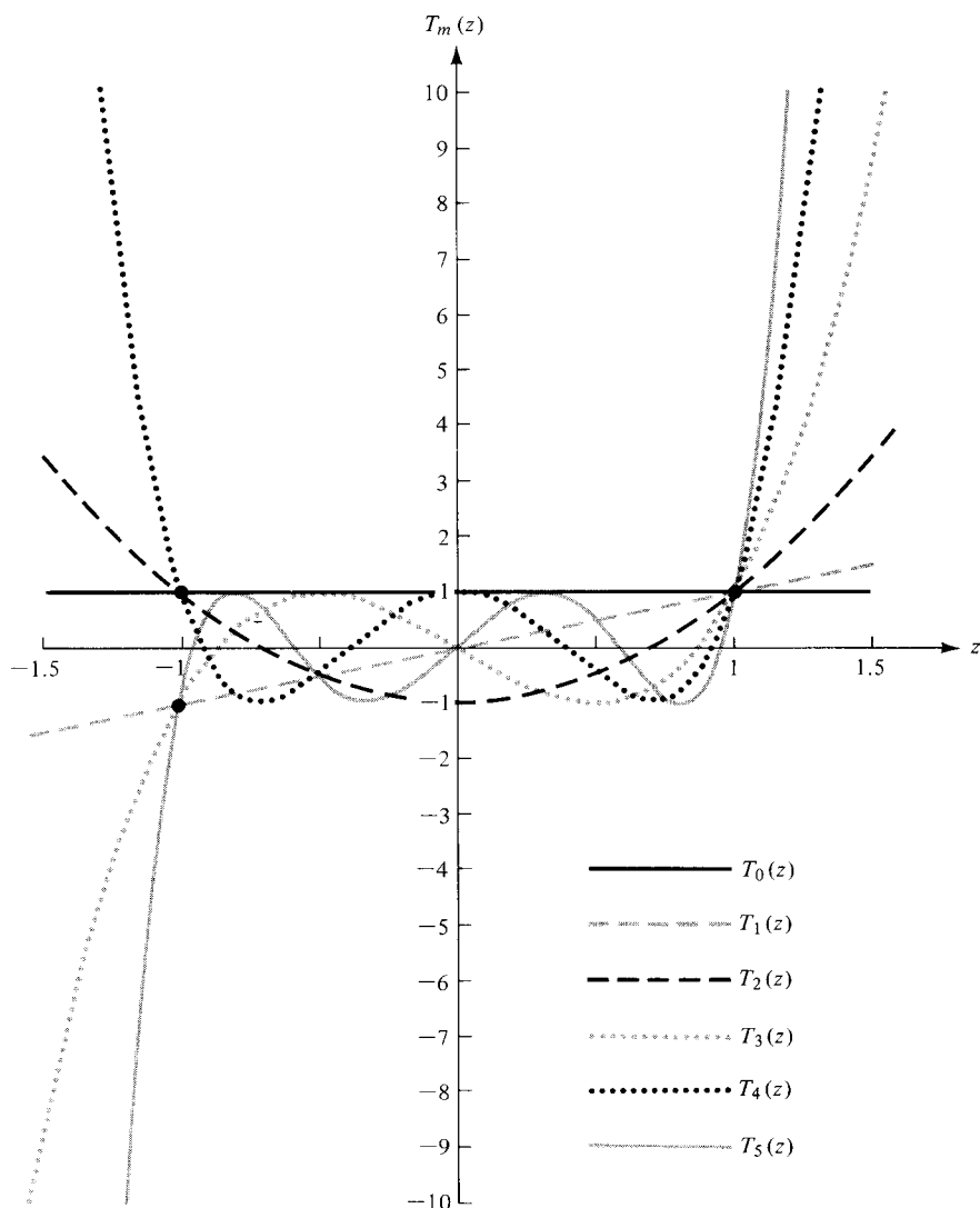
Figure 6.21 Tschebyscheff polynomials of orders zero through five.
