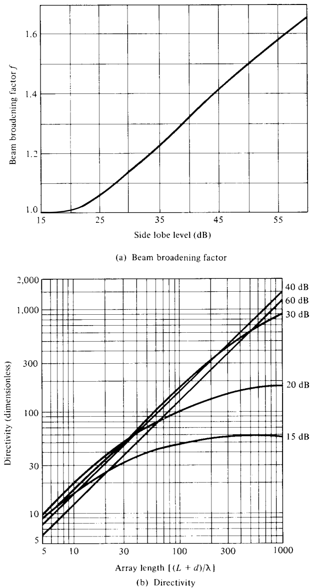
Figure 6.24 Beam broadening factor and directivity of Tschebyscheff arrays. (SOURCE: R. S. Elliott, “Beamwidth and Directivity of Large Scanning Arrays,” First of Two Parts, The Microwave Journal , December 1963).
