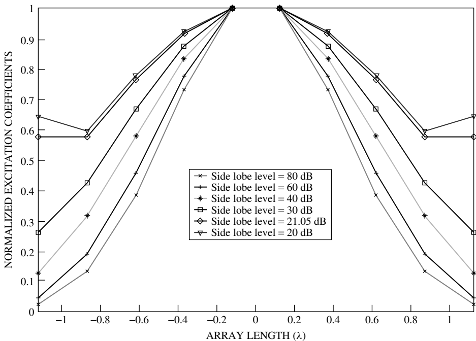
Figure 6.25 Amplitude distribution, for different side lobe levels, of a Dolph-Tschebyscheff array with N = 10 , d = \lambda/4 .
